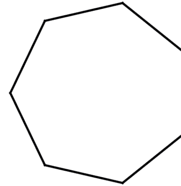
heptagone
