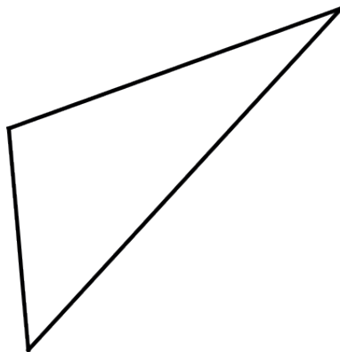
triangle obtusangle
