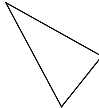
triangle acutangle
