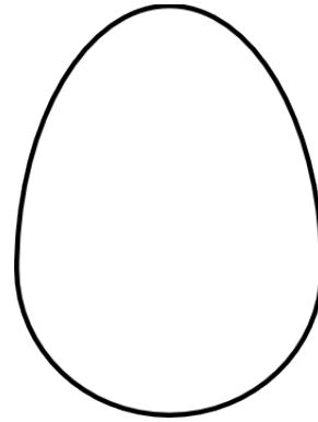
ovale
